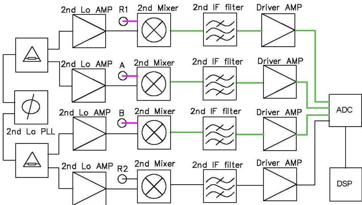
figure2-2: IF block diagram
