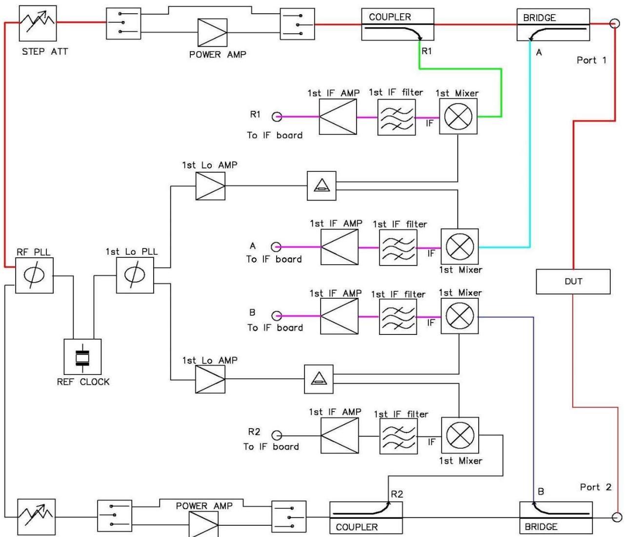
figure2-1: RF block diagram;
