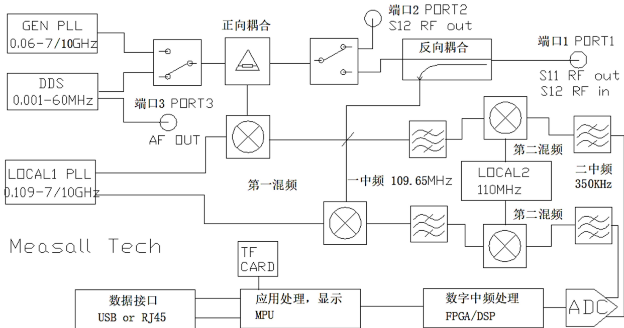
Chart 6-1: KC901M's Schematic Diagram
