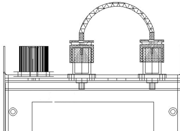
Chart 3-1A: Connect with one cable in calibration
