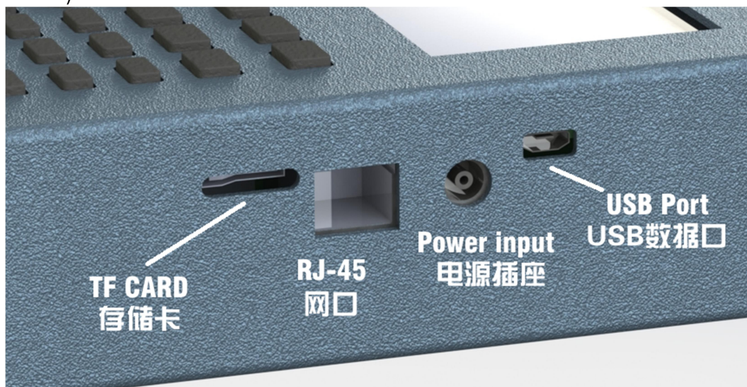
Chart 2-5 Ancillary ports on the right side
