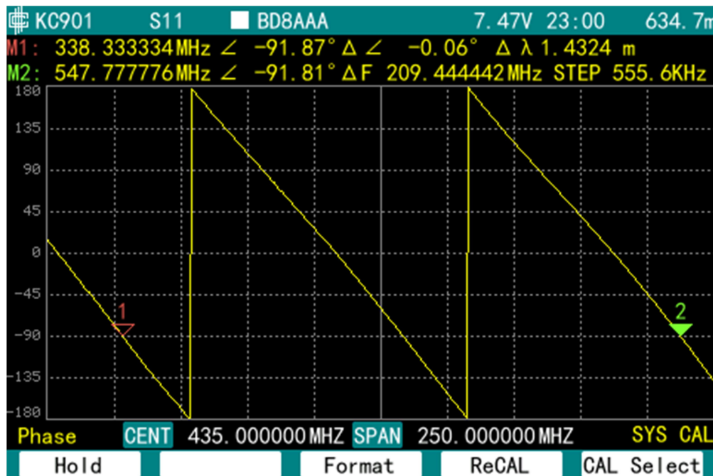
Chart 4-5: Measuring the Cable Electric Length in Phase Frequency Characteristic
